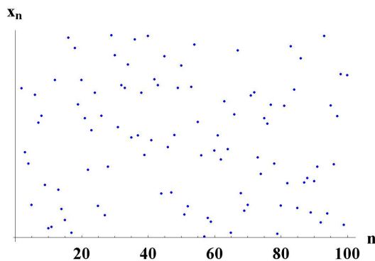
Figure 2: A divergent sequence
