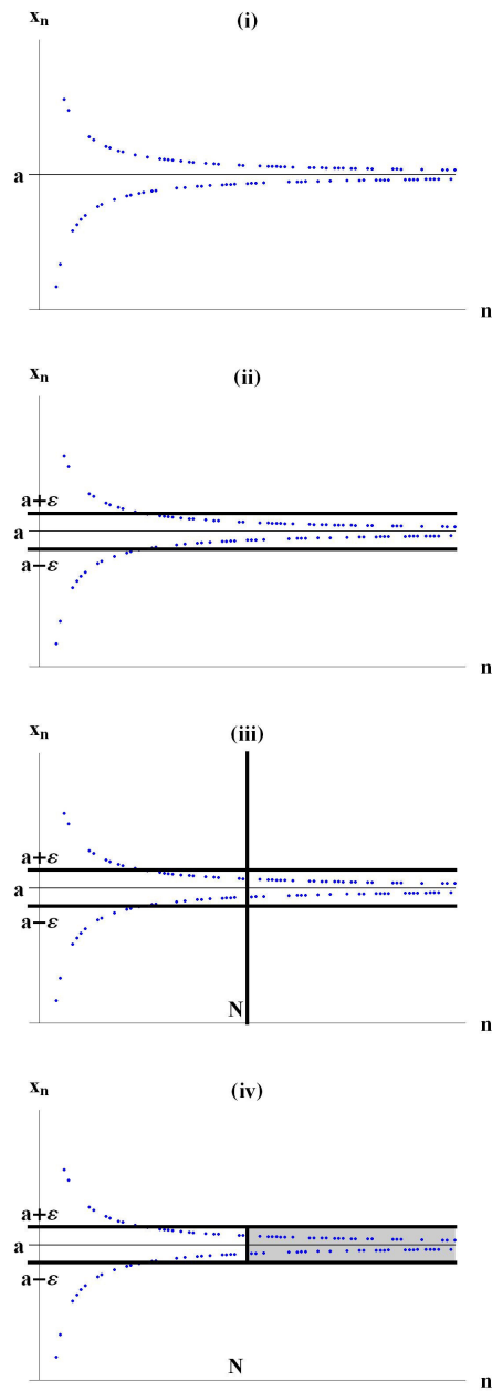
Figure 1: (i) A sequence (x_n) converges to the limit a if ... (ii) ... for all \varepsilon > 0 ... (iii) ... there is an N \in \mathbb{N} , such that ... (iv) ... |x_n - a| < \varepsilon for all n \geq N
