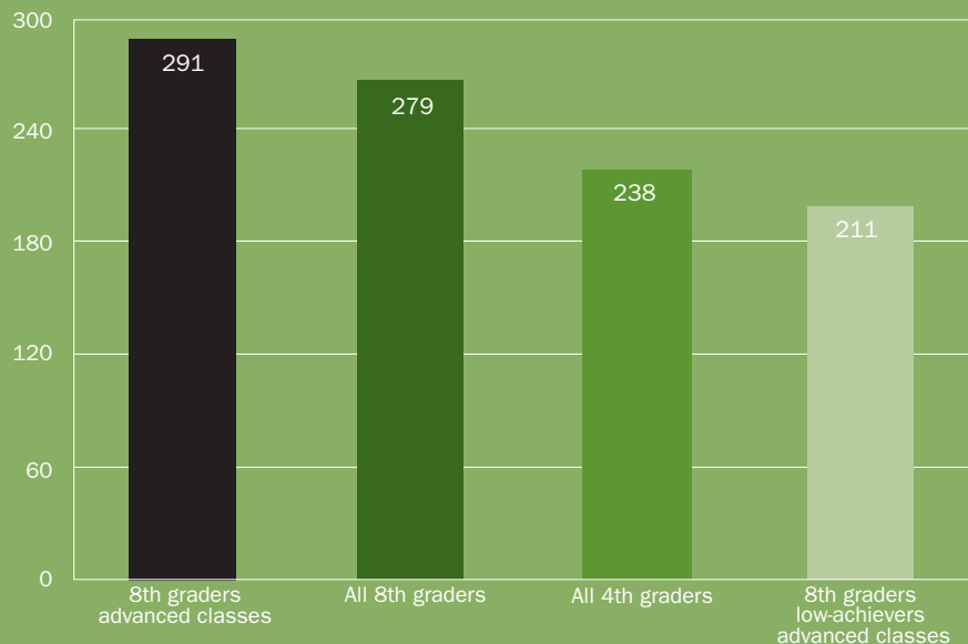
NAEP scores
